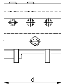
搪孔刀座 Boring bar tool holder
