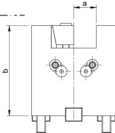
端面刀座 Facing Tool holder
