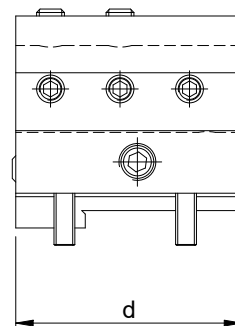
端面刀座 Facing tool holder
