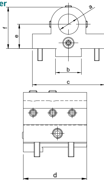
搪孔刀座 Boring bar tool holder
